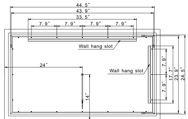
REAR VIEW
