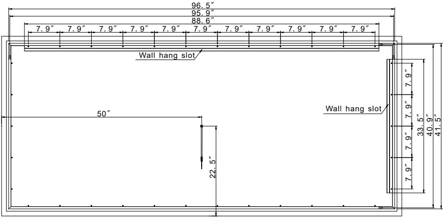
REAR VIEW
