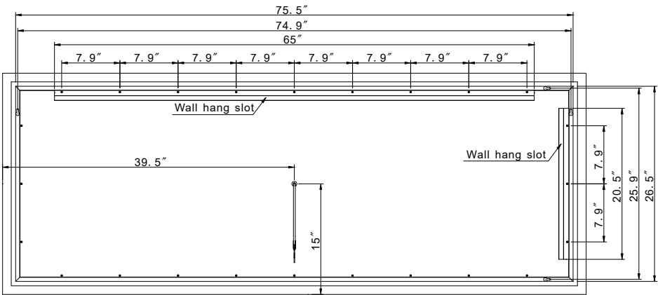
REAR VIEW
