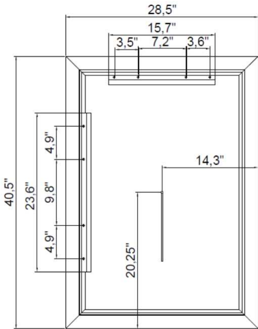
REAR VIEW
