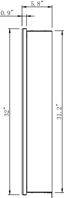
RIGHT SIDE
