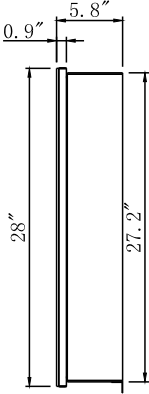
RIGHT SIDE
