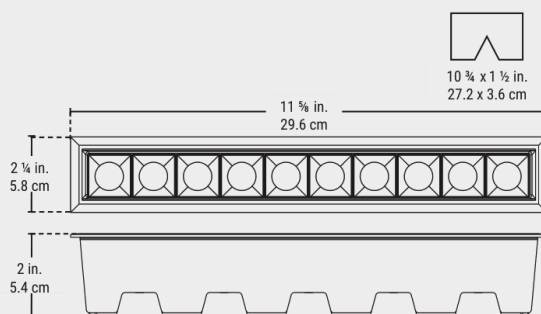
DIMENSIONED DRAWING: LCDL-DISKCB10W (LCDL-DISKCB5W: SAME SECTION, SEE THE TABLE)
