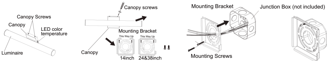
Fig. 1 (left) — fixture, canopy, canopy screws, LED colour temperature, mounting bracket. Fig. 2 (right) — mounting bracket, junction box (not included), mounting screws.
