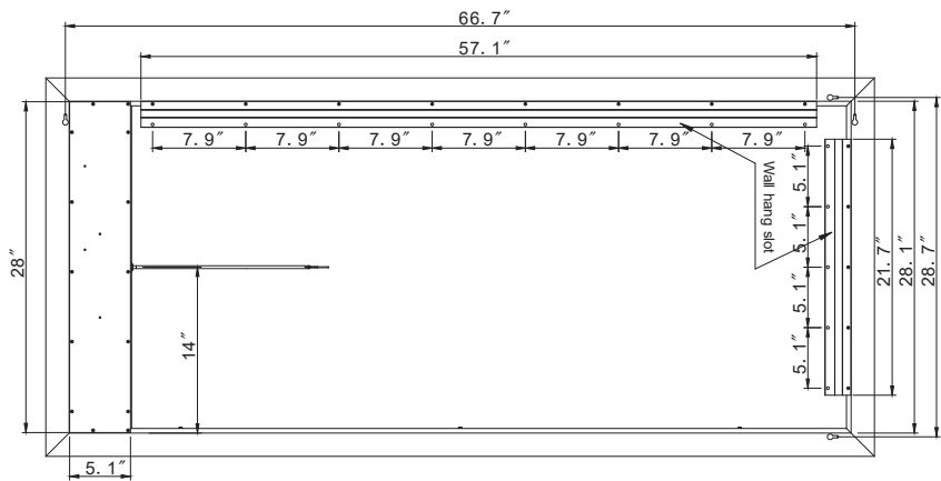
REAR VIEW
