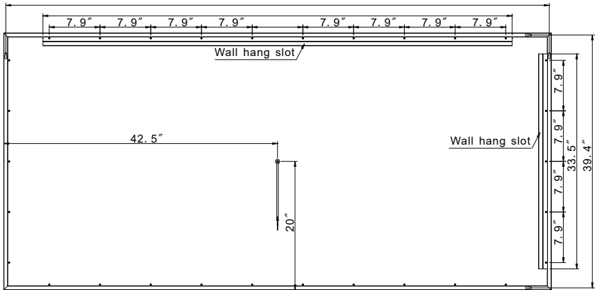
REAR VIEW
