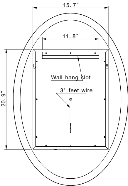
REAR VIEW
