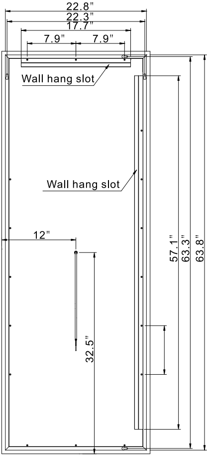
REAR VIEW
